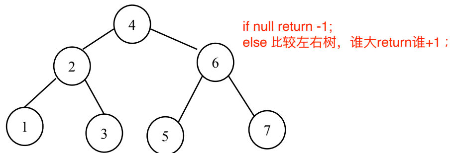
Figure 2: Binary tree
